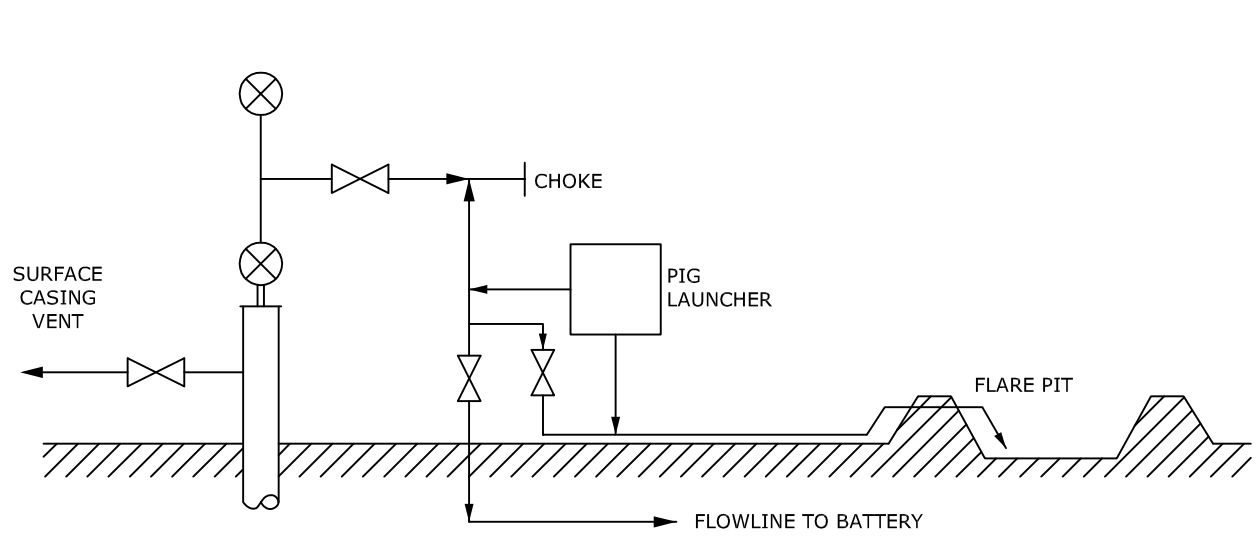
(A) FLOWING WELL TO A BATTERY
