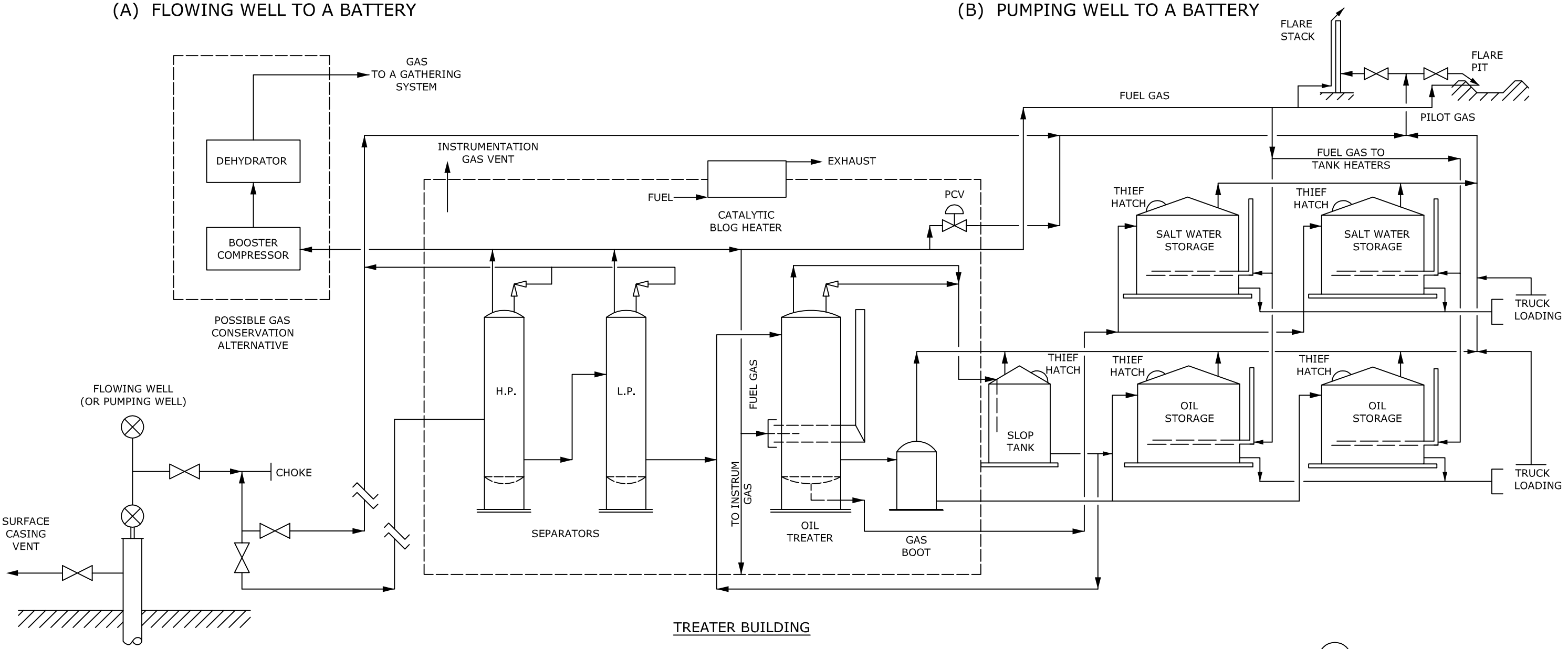
(C) SINGLE-WELL BATTERY (PRODUCTION FACILITIES ON THE WELL SITE)
