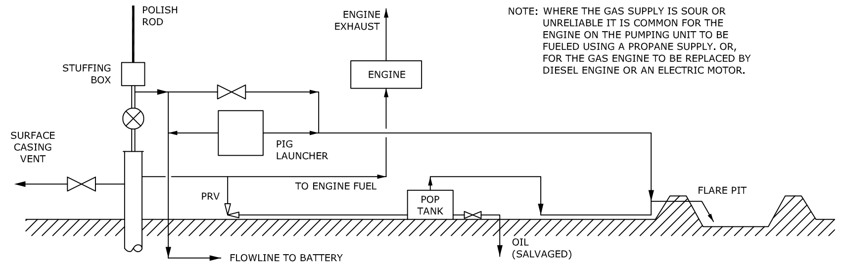
(B) PUMPING WELL TO A BATTERY
